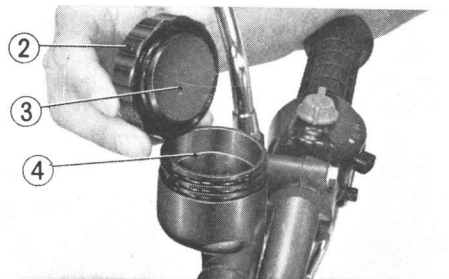
② Reservoir cap ③ Diaphragm
