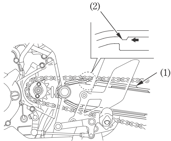
(1) Chain slider
