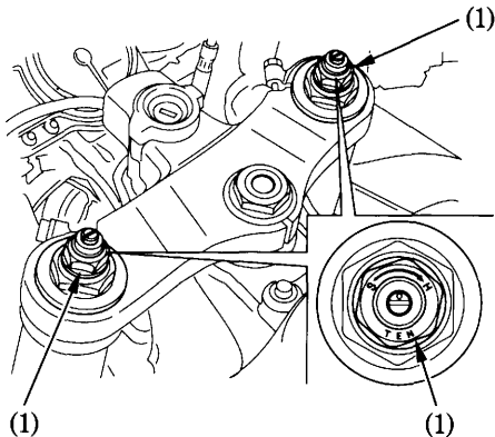
(1) Preload adjuster
