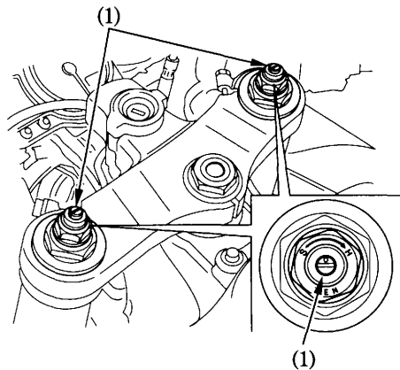
(1) Damping adjuster
