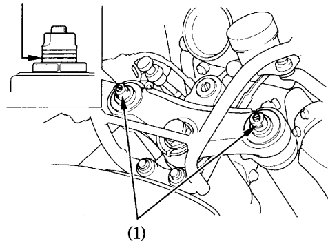
(1) Preload adjuster
