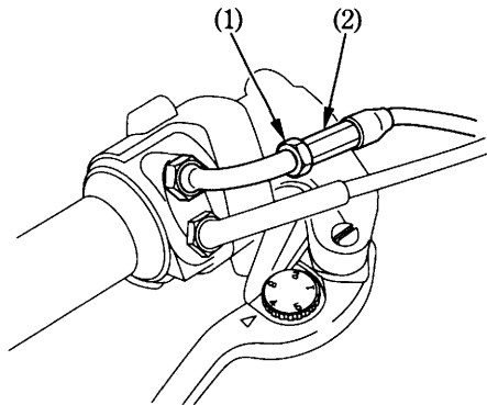
(1) Lock nut
