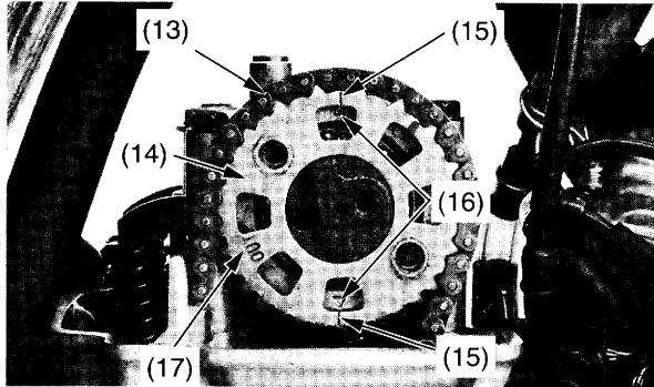
(13) cam chain (14) cam sprocket (15) timing marks (16) "Δ" marks (17) "OUT" mark
