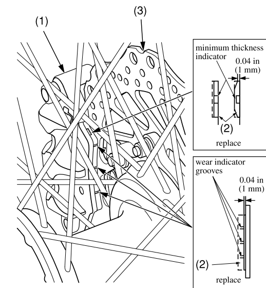
(1) front brake caliper (2) brake pads (3) brake disc
