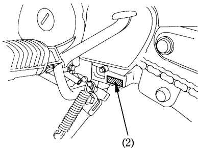
(2) Engine number
