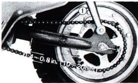
1 Drive chain
