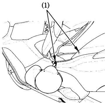
(1) Holder hooks
