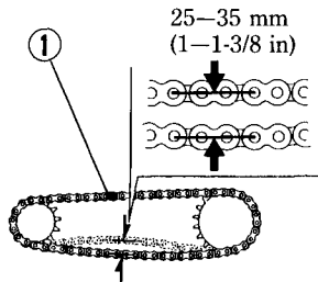
(1) Drive chain
