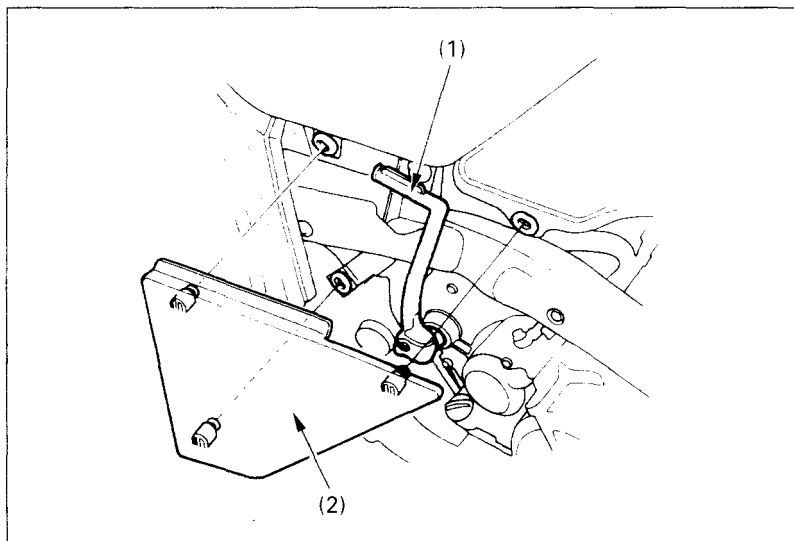
Fig. 2-9 (1) Kick starter
