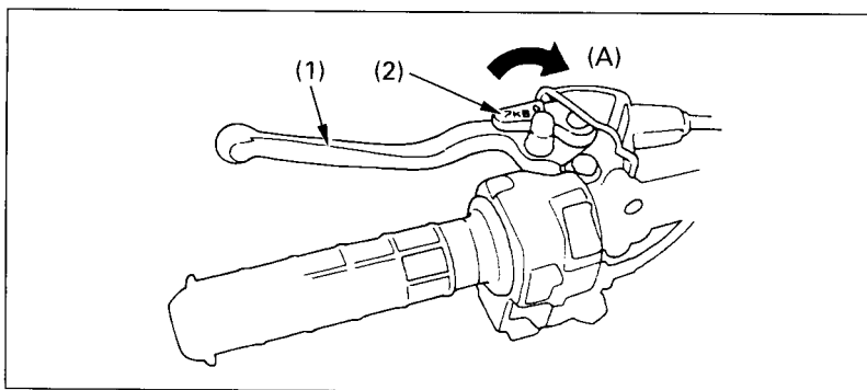
Fig. 2-21 (1) Rear brake lever/ Parking brake lever (2) Lock lever (A) To lock
