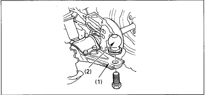
Fig. 2-22 (1) Trailer hitch (2) An example ball
