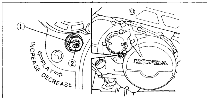
Fig. 4-16 (1) Lock nut
