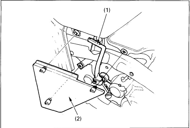
Fig. 2-9 (1) Kick starter
