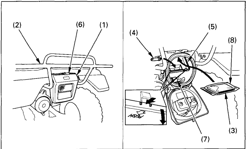
Fig. 2-31 (1) Storage compartment (2) Rear cargo rack (3) Owner's manual (4) Air pressure gauge
