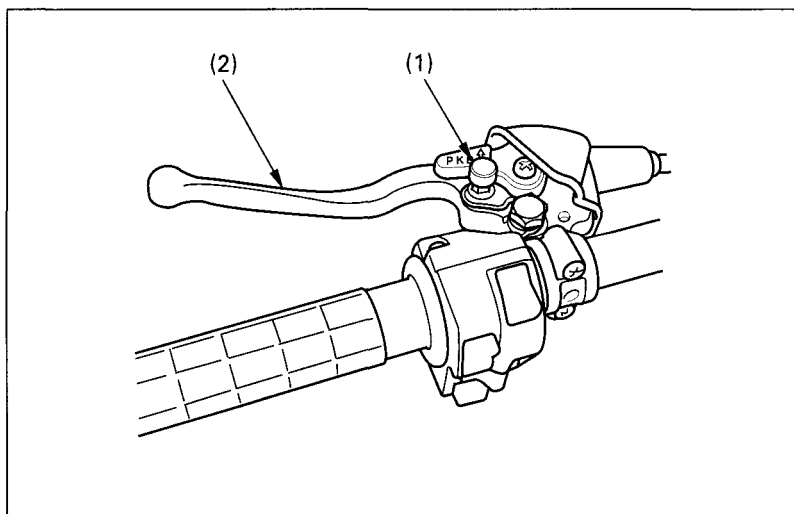
Fig. 2-22 (1) Reverse selector knob (2) Rear brake lever
