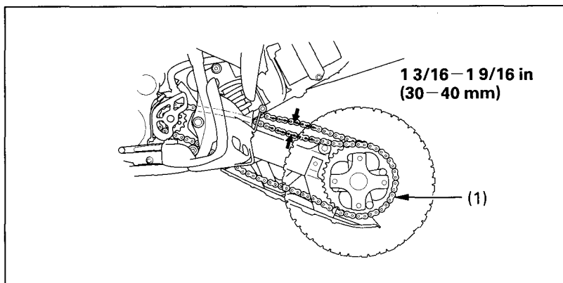
Fig. 4-15 (1) Drive chain
