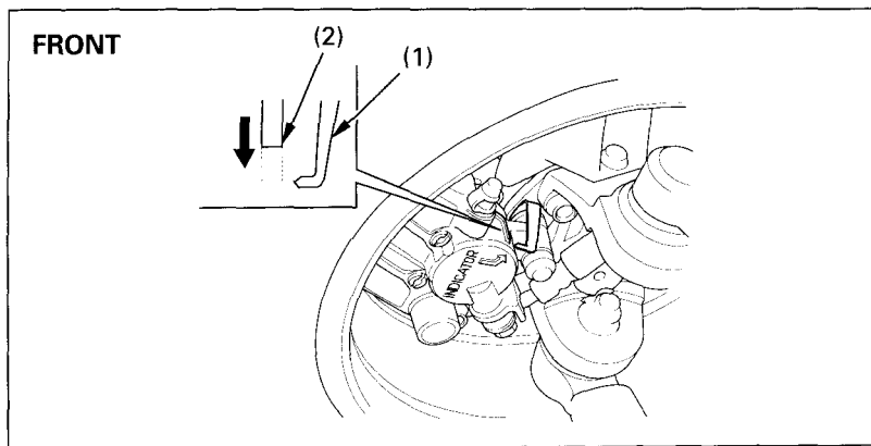
Fig. 4-26 (1) Wear indicator
