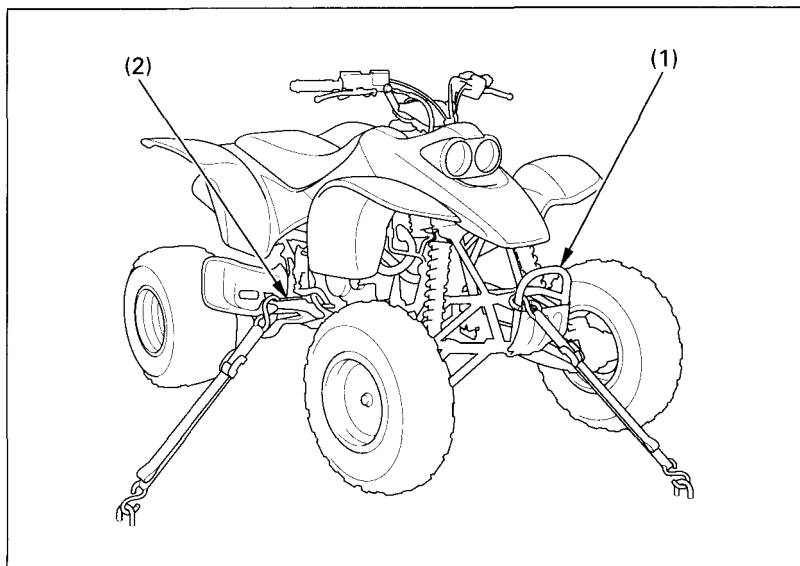
Fig. 4-37 Points to secure Sportrax with tie downs
