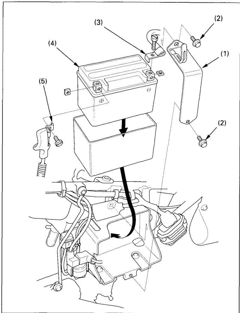
Fig. 4-21 (1) Battery holder (2) Mount bolts (3) Negative (-) terminal lead
