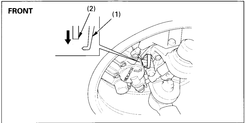
Fig. 4-25 (1) Wear indicator
