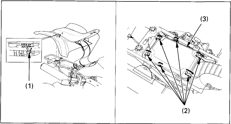
Fig. 4-5 (1) Seat lock lever
