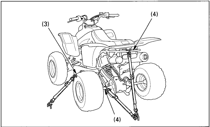
Fig. 4-38 Points to secure FOURTRAX with tie downs (3) Left footpeg (4) Rear carry pipe or Rear axle shaft
