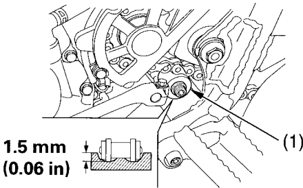
(1) chain roller
