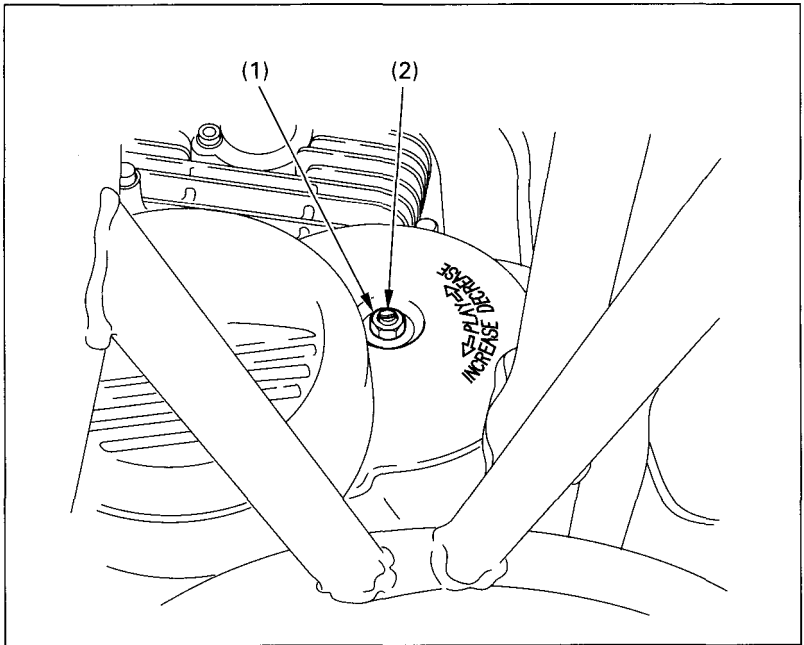
Fig. 4-17 (1) Lock nut
