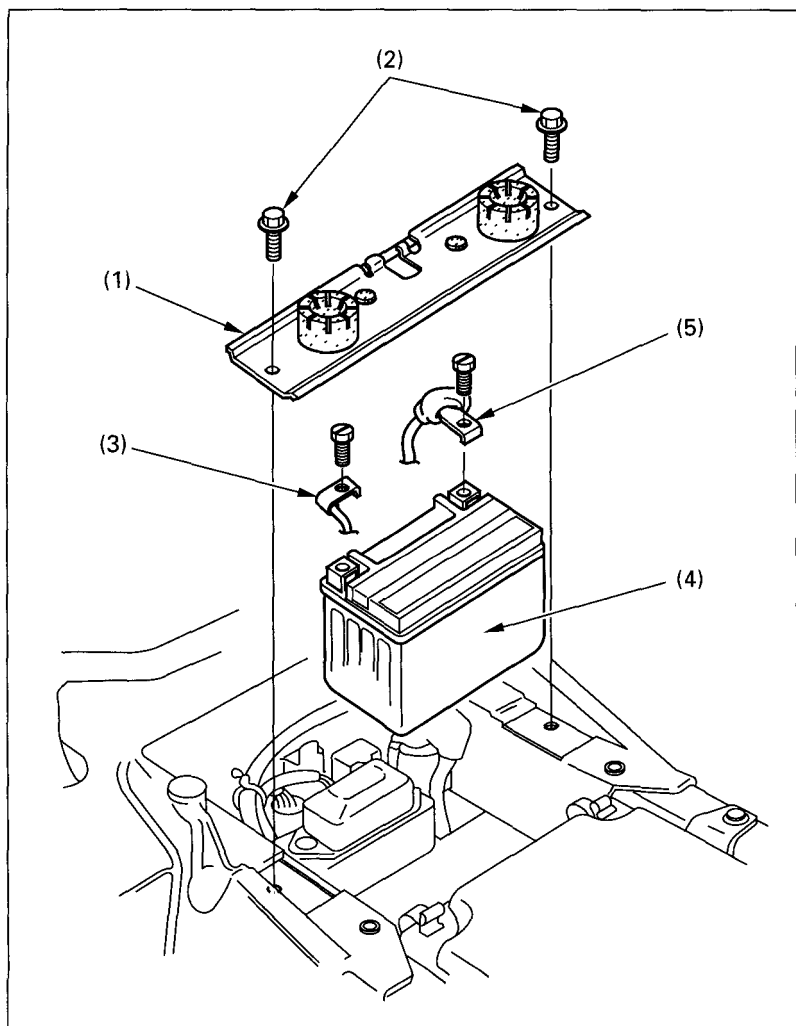
Fig. 4-19 (1) Battery holder (2) Mount bolts (3) Negative (-) terminal lead
