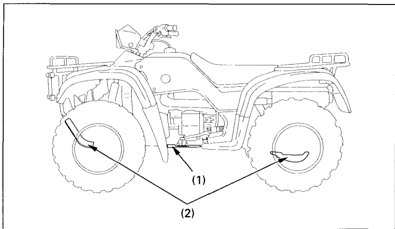
Fig. 4-37 (1) Engine guard
