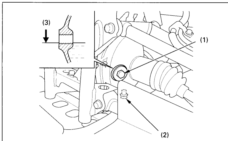
Fig. 4-17 (1) Oil filler cap (3) Lower edge of inspection hole (2) Oil drain plug
