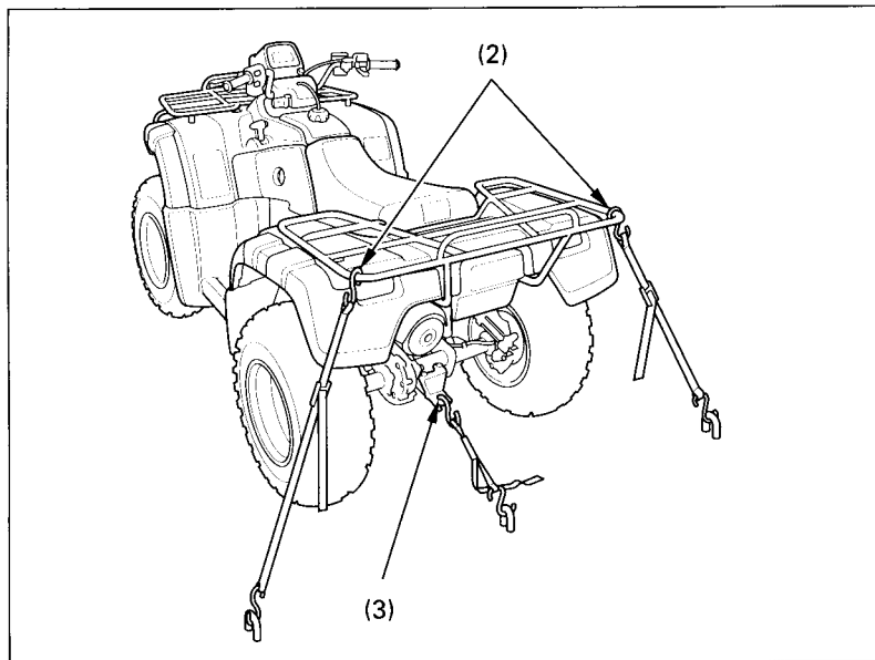
Fig. 4-45 Points to secure FOURTRAX with tie downs
