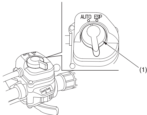
(1) drive mode select switch
