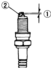
(1) Spark plug gap (2) Side electrode
