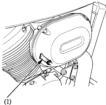
(1) Drain tube
