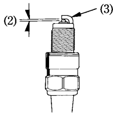
(3) Side electrode
