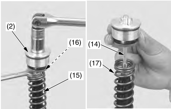
(2) fork cap (14) adjuster needle rod (15) piston rod (16) lock nut (17) fork spring
