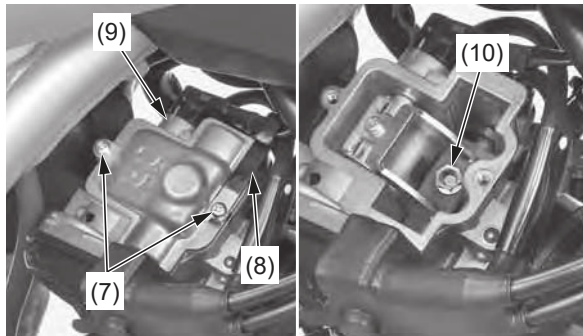
(7) carburetor top screws (9) carburetor top (8) cable clamp (10) jet needle/holder assembly
