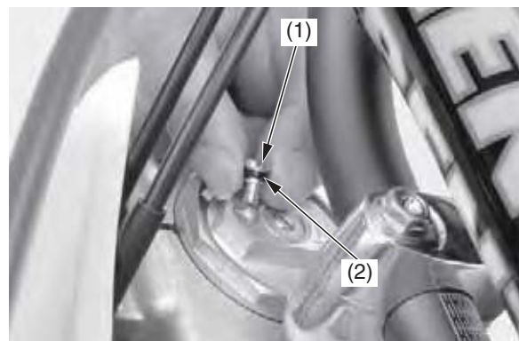
(1) pressure release screw (2) O-rings
