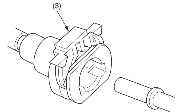
(3) slide retainer
