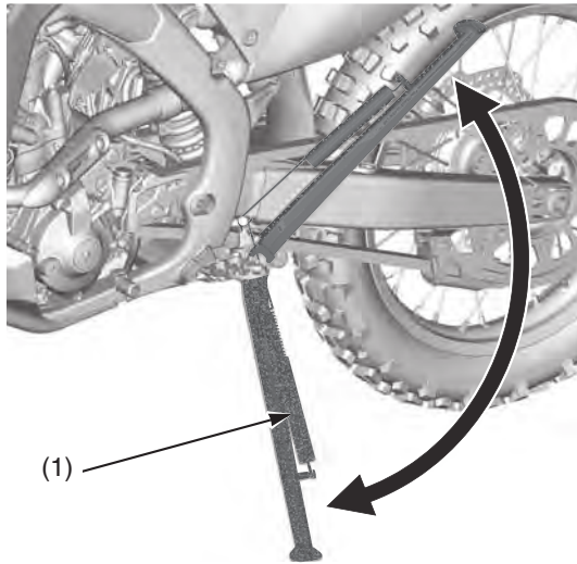
(1) side stand spring
