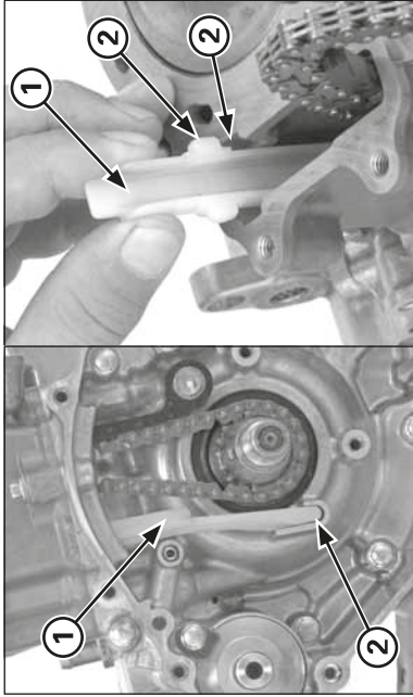
(1) CAM CHAIN GUIDE (2) ALIGN
