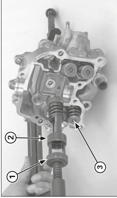
(1) VALVE SPRING COMPRESSOR (2) ATTACHMENT (3) COTTERS
