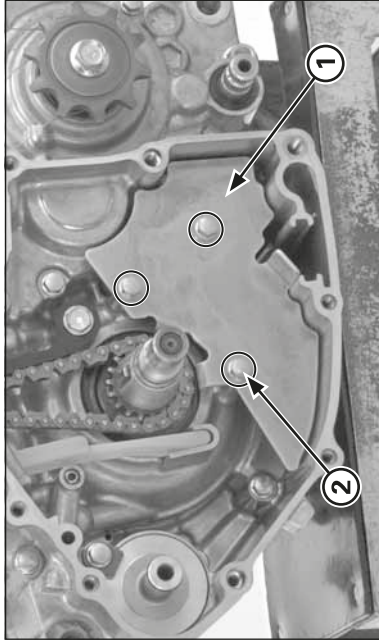
(1) CAM CHAIN GUIDE PLATE (2) BOLTS
