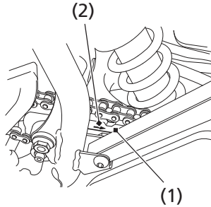
(1) drive chain slider (2) wear limit line
