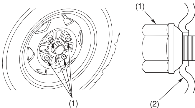
(1) wheel nuts
