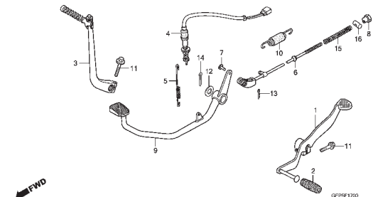
C-17 Pedal de Partida • Pedal de Freio / Kick Started Arm • Pedal / Brazo Arranque de Pie • Pedal
