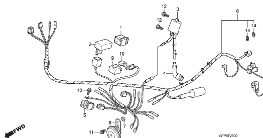
C-26 Fiação Principal / Wire Harness / Alambreaje Principal
