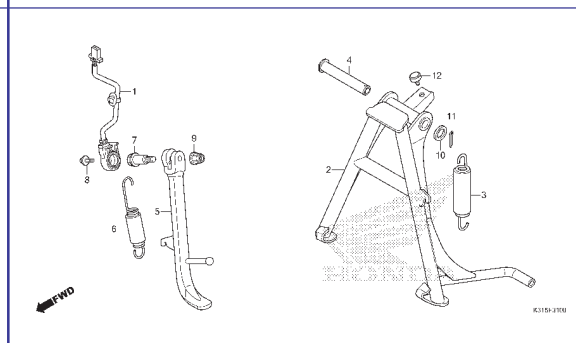
C-31 Cavalete
