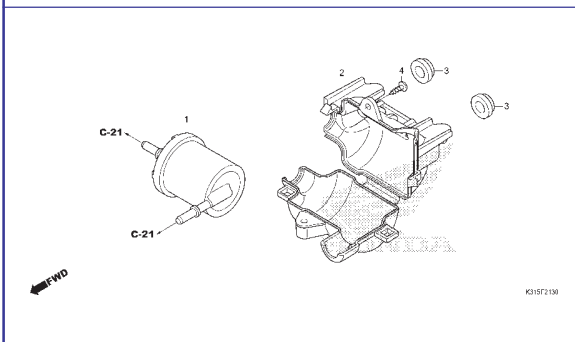
C-24 Tampa Lateral • Rabeta
