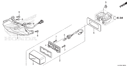
C-39 Chassi
