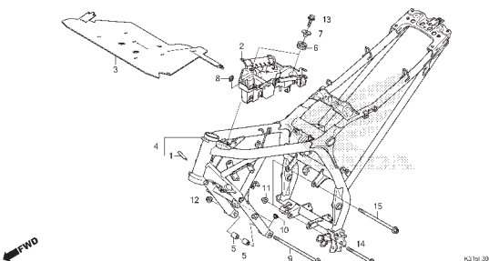
C-39 Chassi
